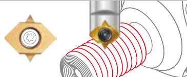
D Gooving
