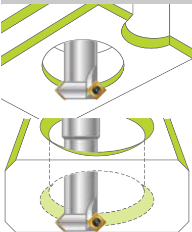
Backward Circular Chamfering
